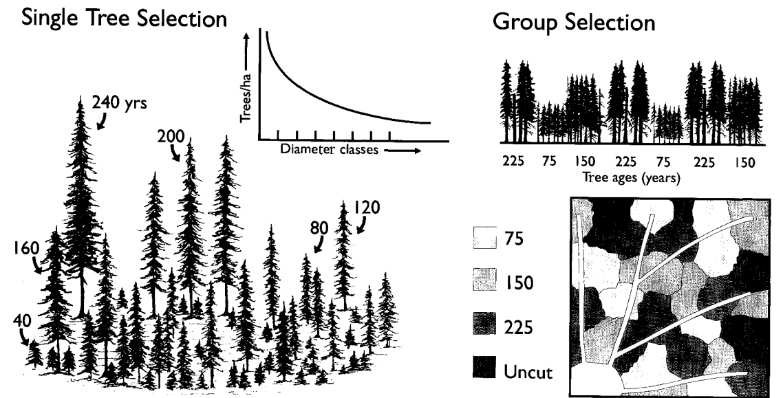
Fig. 1. Examples of silvicultural systems suited to maintaining the stand characteristics required by caribou (Stevenson et al. , 1994).
