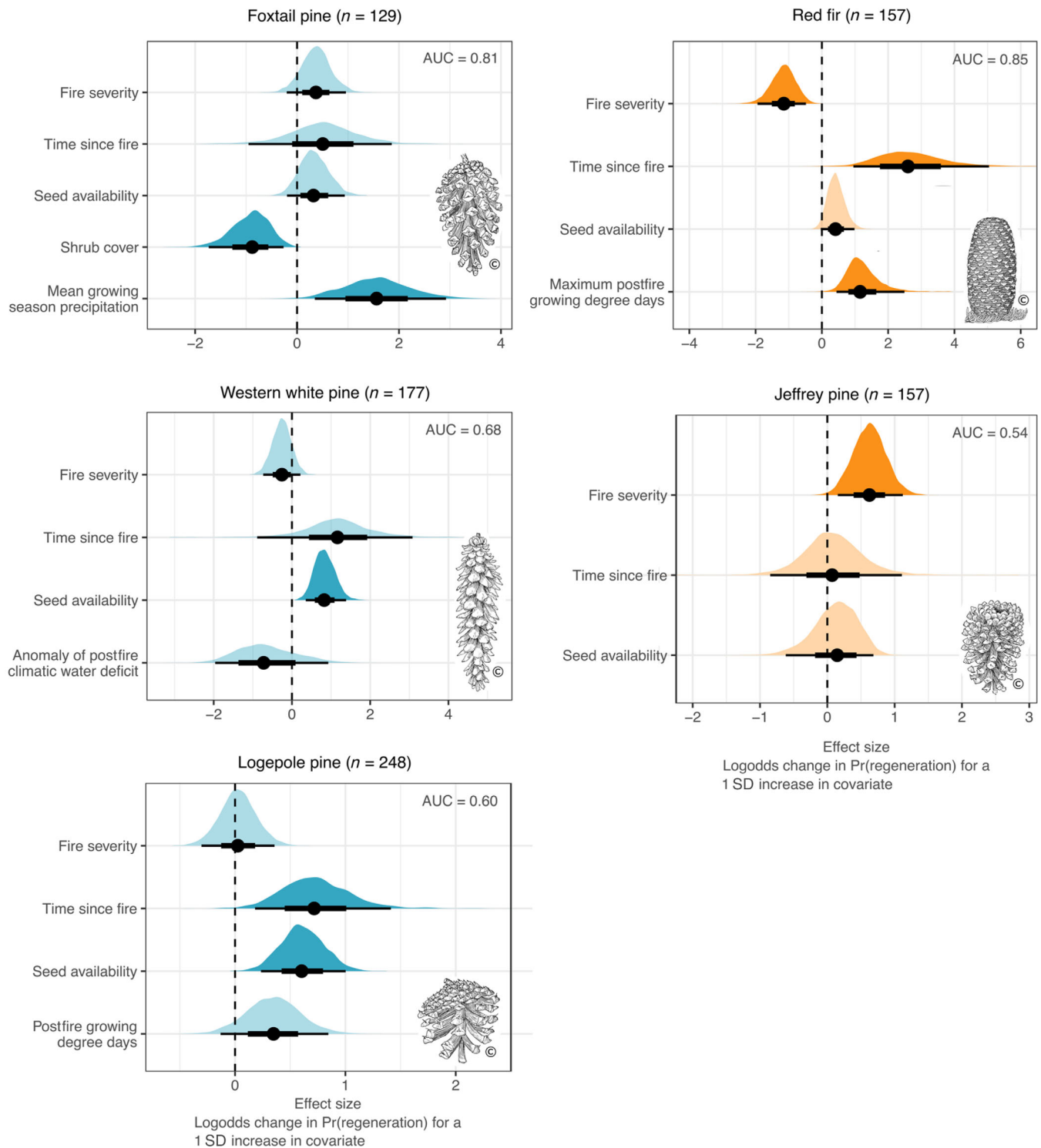
FIGURE 3 Plots showing the effect size of predictors on \Pr(\text{regeneration}) for foxtail pine, western white pine, lodgepole pine, red fir, and Jeffrey pine in subalpine forest. \Pr(\text{regeneration}) is the probability that a 60 m 2 plot (405 m 2 for Jeffrey pine) contains at least one postfire seedling (seedling of any age for Jeffrey pine). Black dots and bars show model-estimated means with 80% and 95% confidence interval (CI), respectively. Shading shows distribution of the mean, with darker shading indicating that the 95% CI does not cross zero. Blue shading represents subalpine species, and orange shading represents montane species. AUC, area under the receiver operating curve, a measure of model classification accuracy (range 0–1). Drawings from the Jepson eFlora (Jepson Flora Project eds., 2021, [ https://ucjeps.berkeley.edu/eflora/ ]) Regents of the University of California, used with permission.
